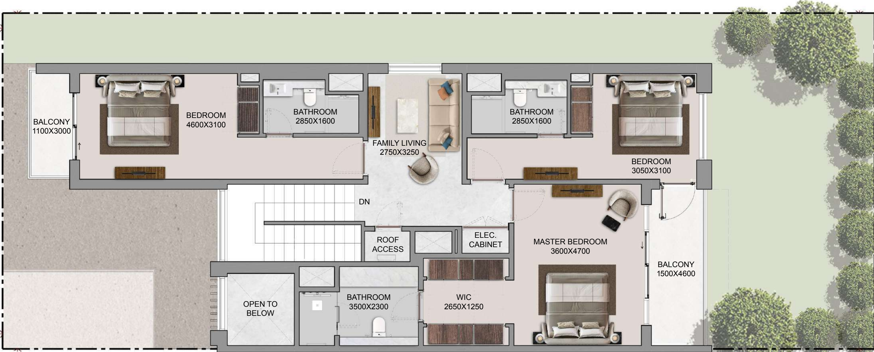
FIRST FLOOR
