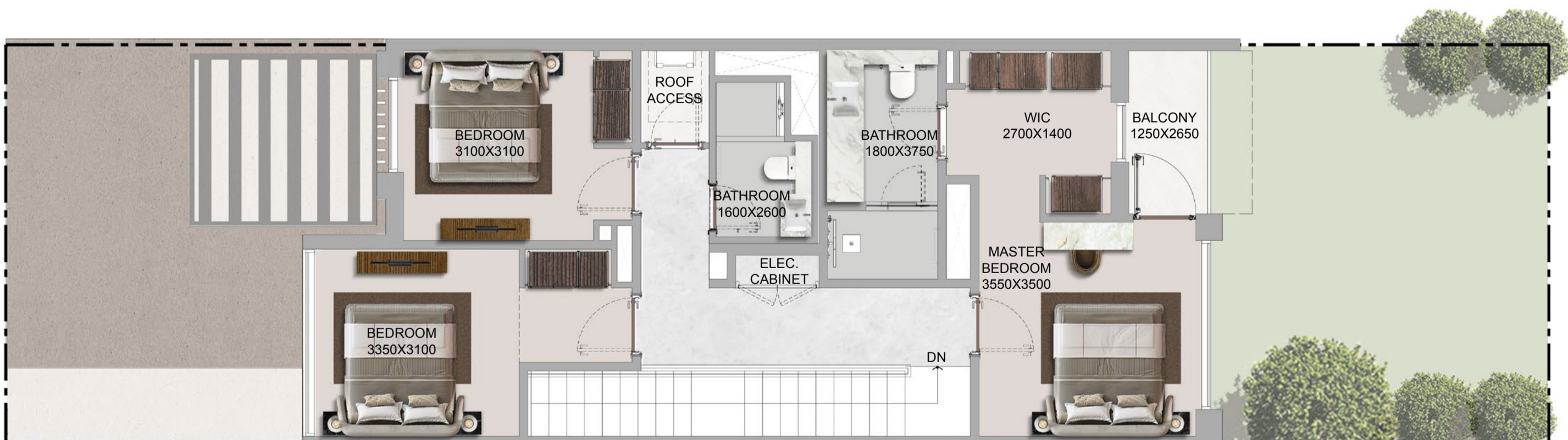
FIRST FLOOR
