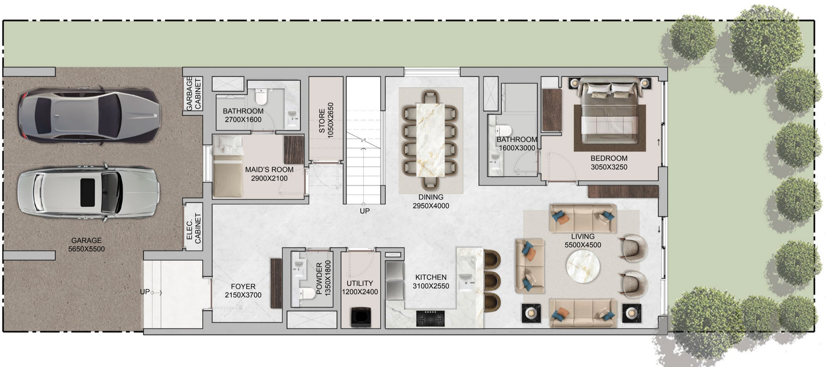
GROUND FLOOR
